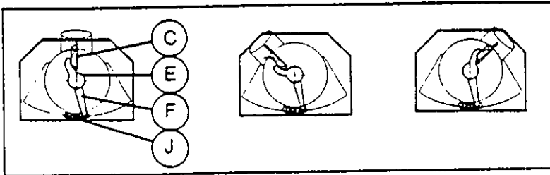
Fig. 5b Damper mechanism for various flue orientations
